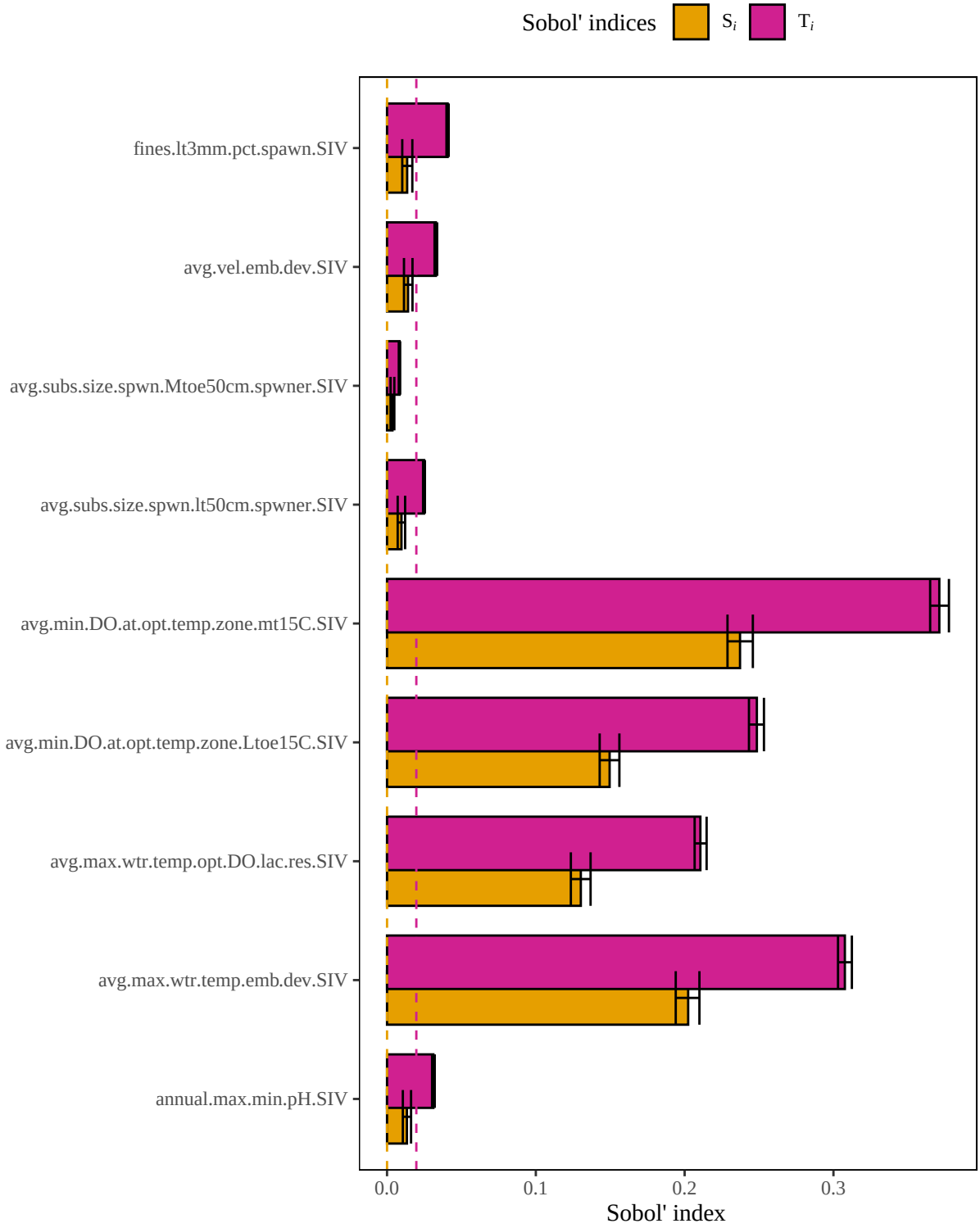
Figure 3. Results of a sensitivity analysis for the rainbowtroutLac model based on the original author-specified model outlined in Raleigh et al. (1984). Dashed lines represent baseline numerical approximation error for S_i and T_i ( i.e. , dummy variables).
