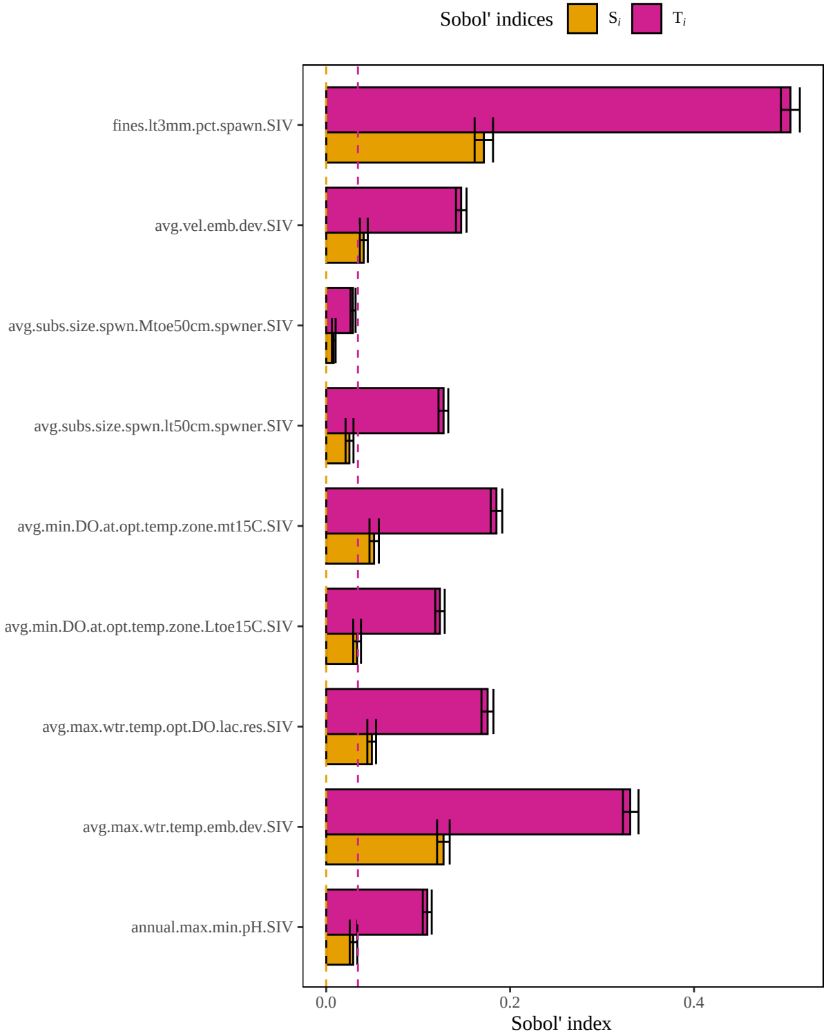
Figure 6. Results of a sensitivity analysis for the rainbowtroutLac model based on a limiting factor structure. Dashed lines represent baseline numerical approximation error for S_i and T_i ( i.e. , dummy variables).
